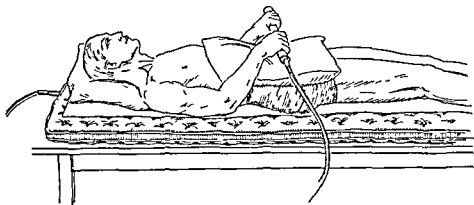
FIG 76 Autocondensation
