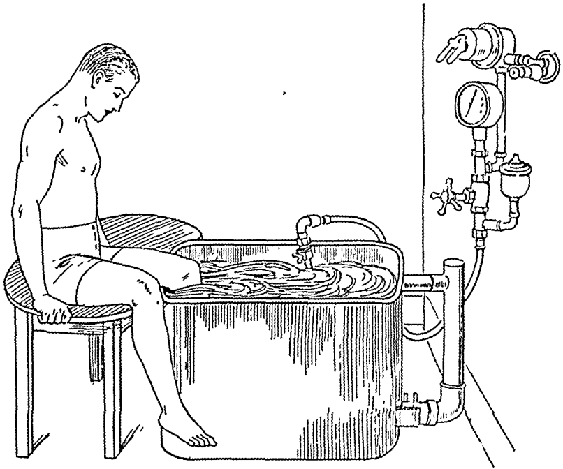
FIG. 20. Leg whirlpool bath. Ejector type.
