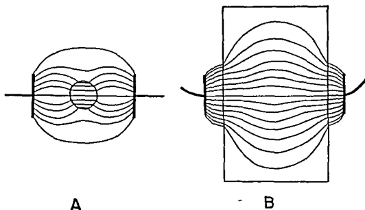
FIG 79 Current flow with air spaced electrodes (schematic) A Electrodes are large in relation to object B Electrodes are small in relation to object (Bierman W Medical Applications of the Short Wave Current. Courtesy of Williams & Wilkins Company)
