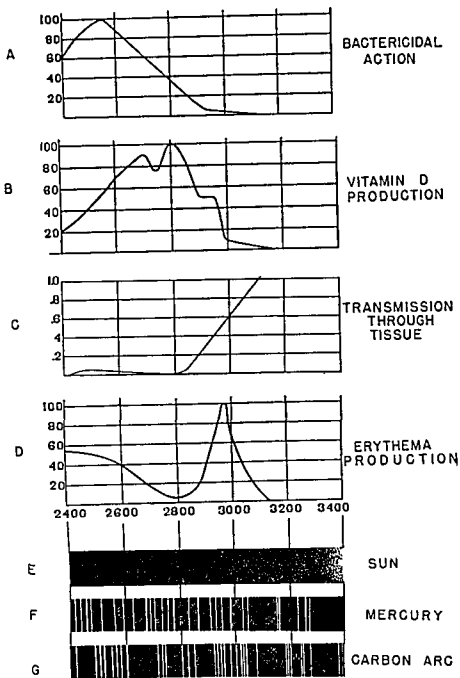
FIG. 169 Biological effects of ultraviolet radiation between 2400 and 3400 A Spectral distribution of ultraviolet radiation from the sun hot quartz mercury arc and carbon arc within the same limits
