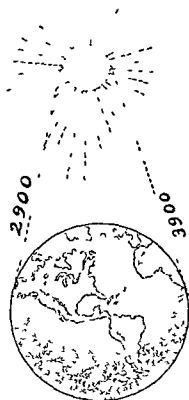
FIG. 163. The limits of solar ultraviolet radiation reaching the earth's surface indicated in Angstrom units.
